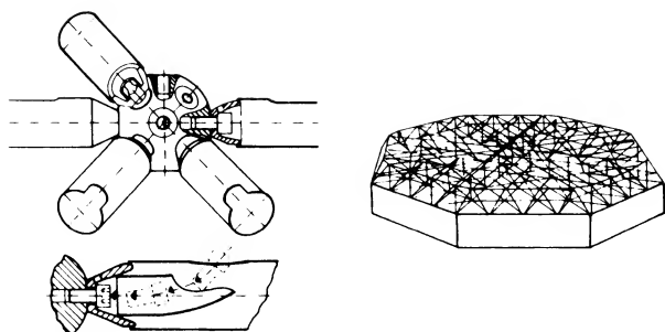
① Joint
